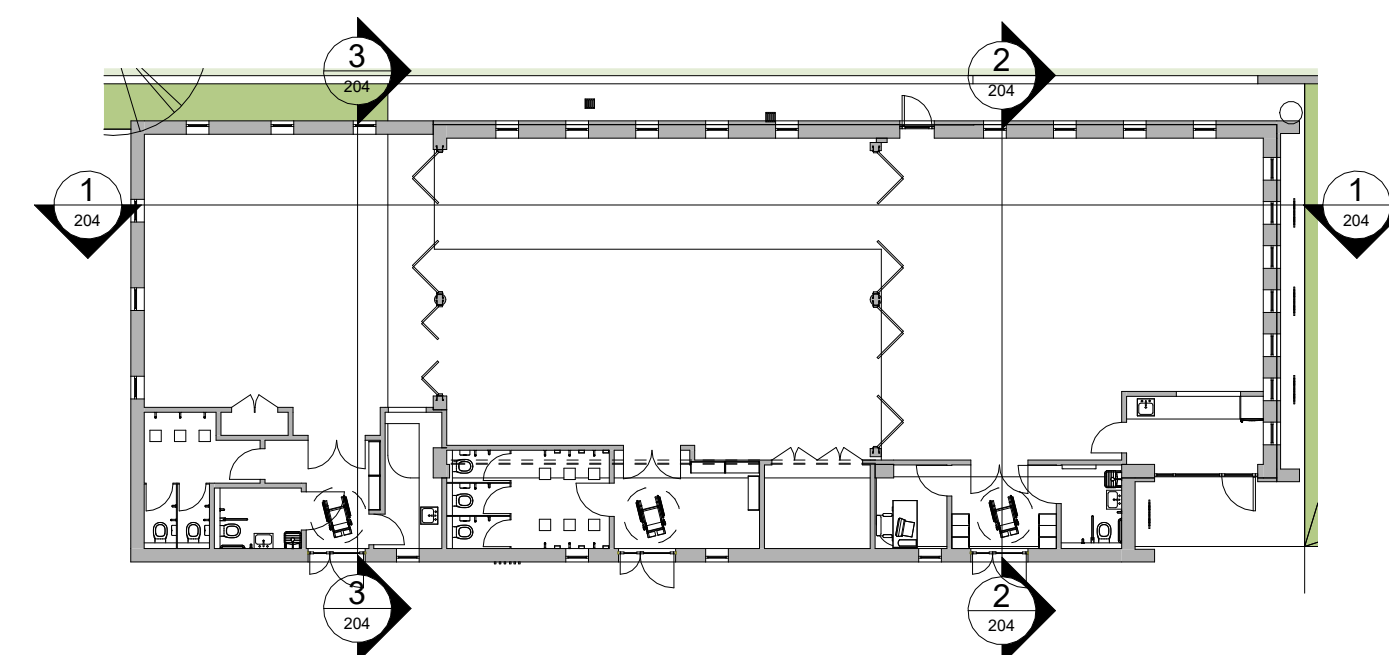
4 Key - Proposed Ground Floor Plan 1 : 200
