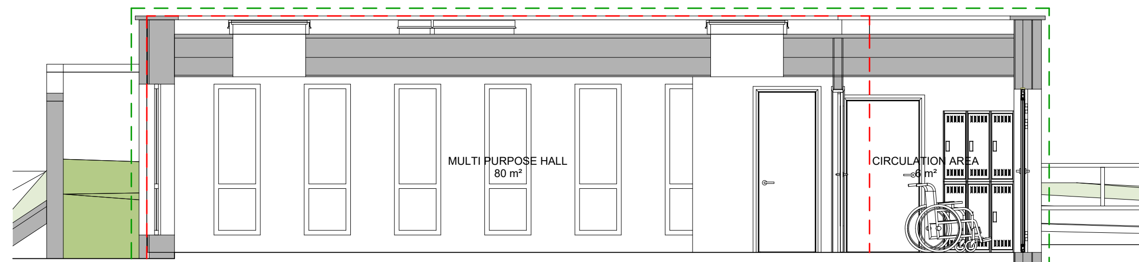
2 Proposed Section 10 1 : 50
