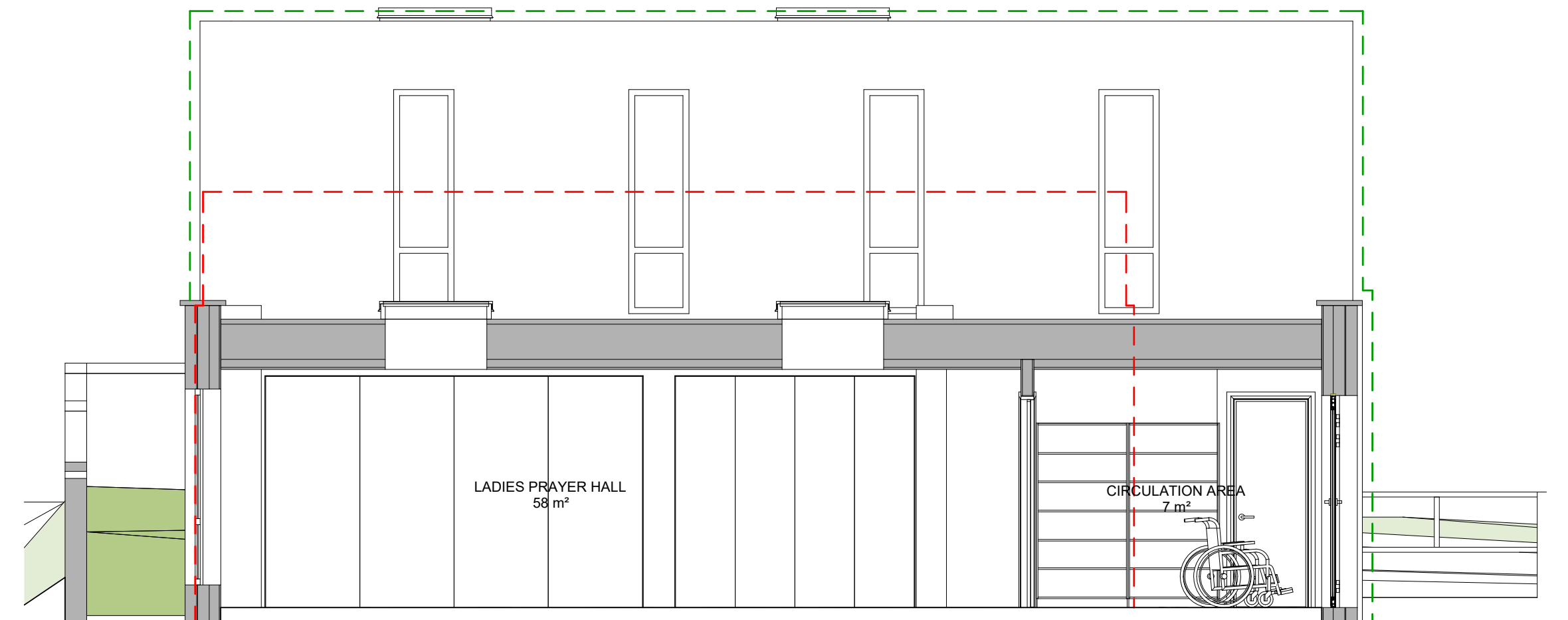
3 Proposed Section 11 1 : 50
