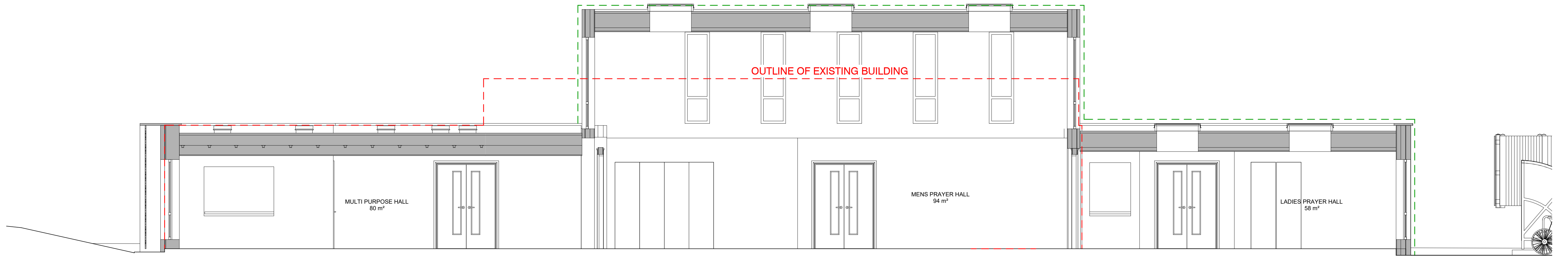
1 Proposed Section 9 1 : 50
